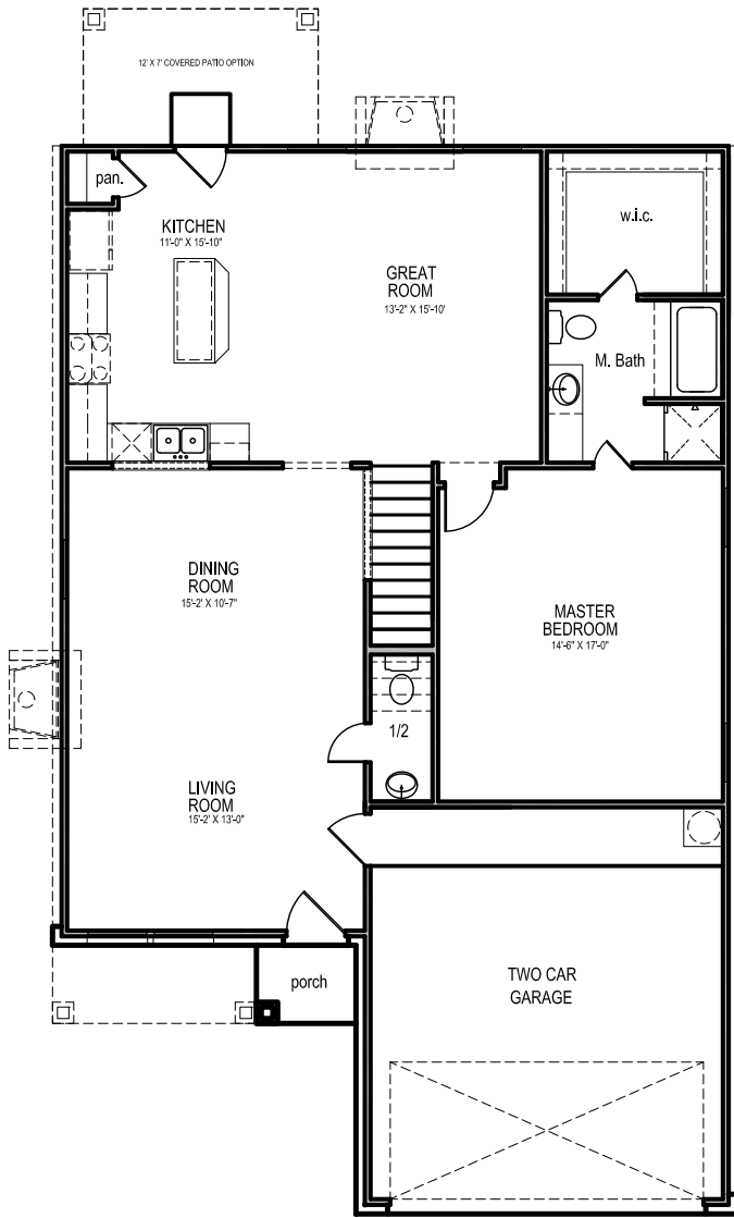
1ST FLOOR
