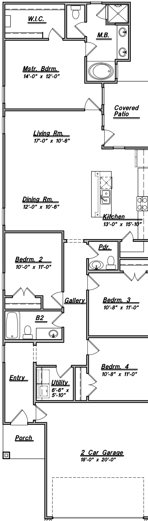
FLOOR PLAN Plan 1688
