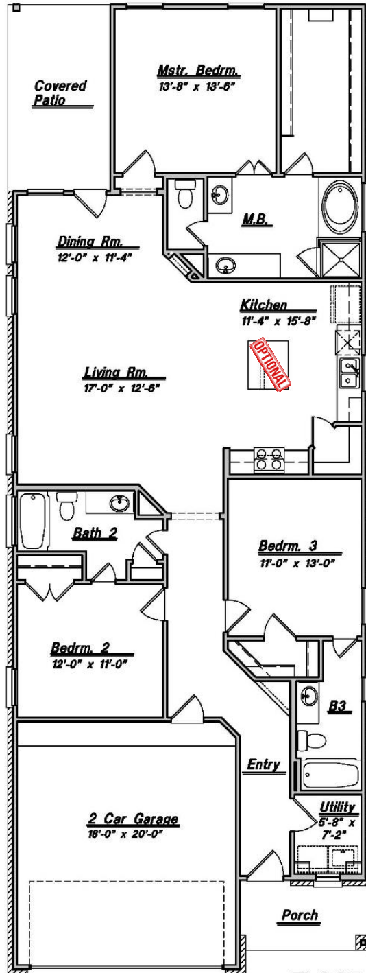
FLOOR PLAN Plan 1784
