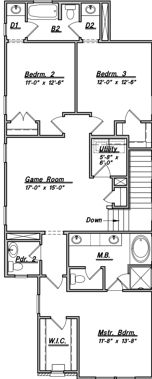
SECOND FLOOR PLAN Plan 2108
