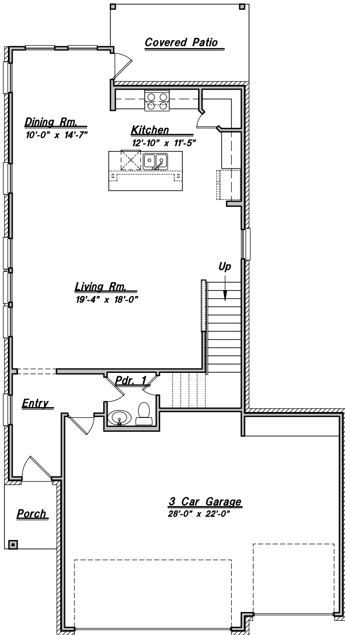
FIRST FLOOR PLAN Plan 2108
