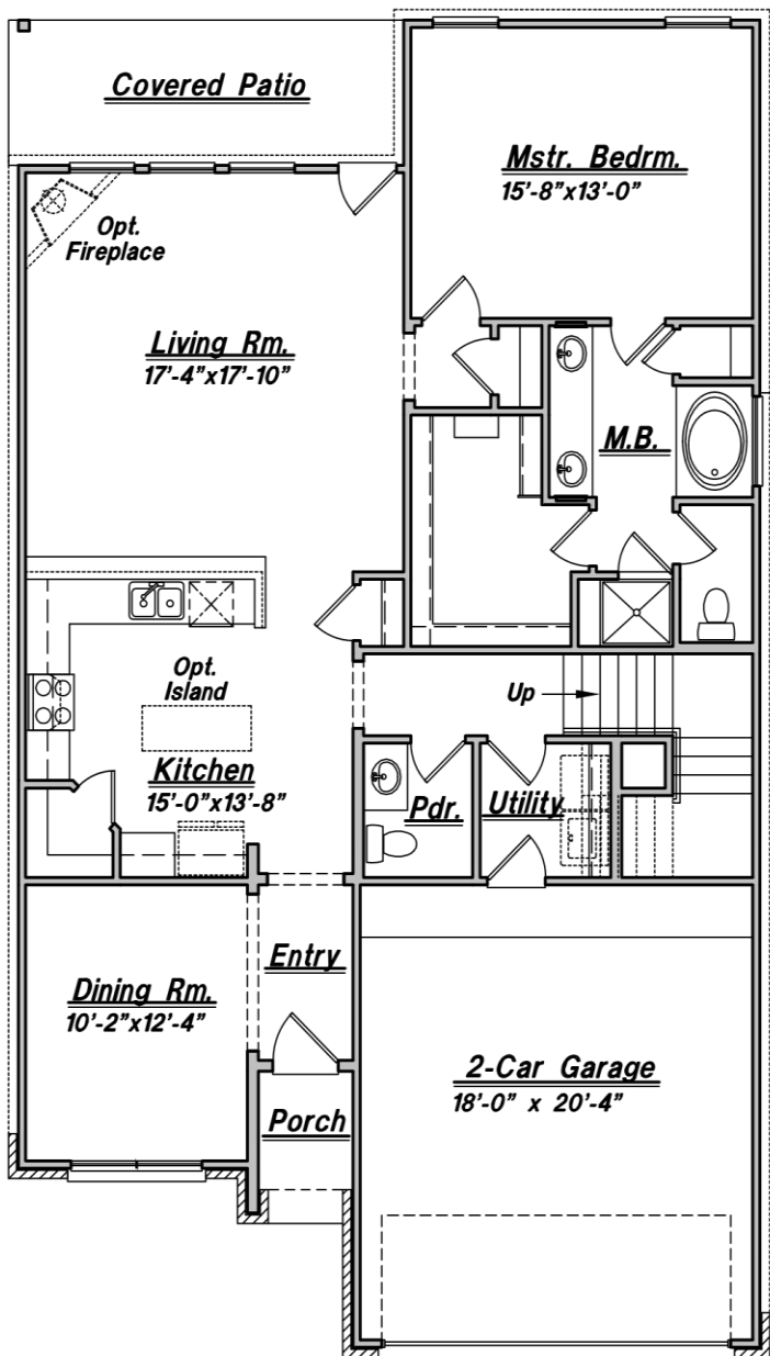
FLOOR PLAN Plan 2123
