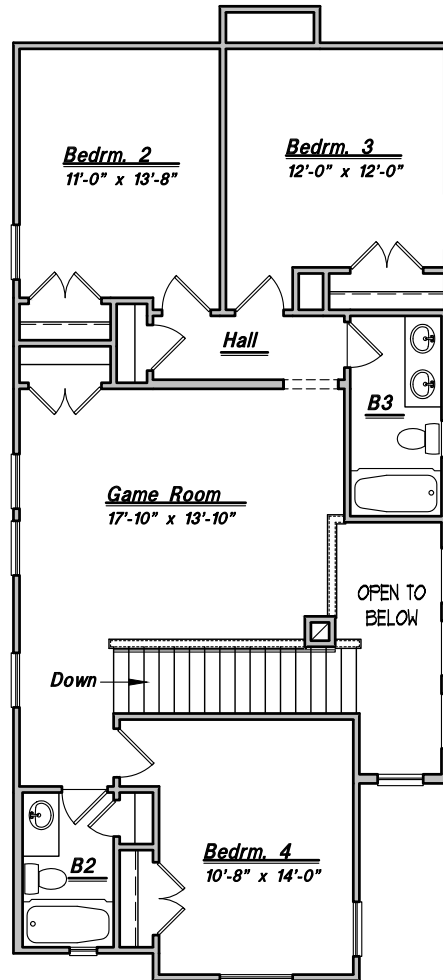
SECOND FLOOR Plan 2253
