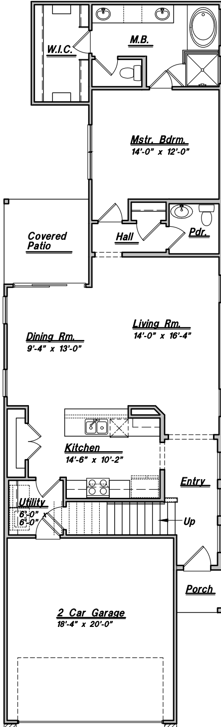
FIRST FLOOR Plan 2253
