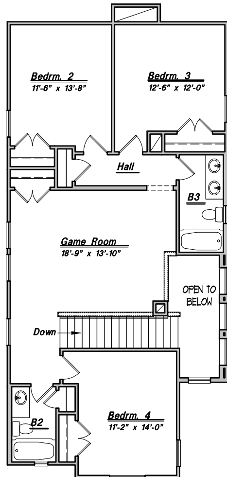
SECOND FLOOR Plan 2253
