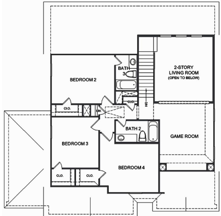
SECOND FLOOR PLAN PLAN 2365 3-CAR GARAGE
