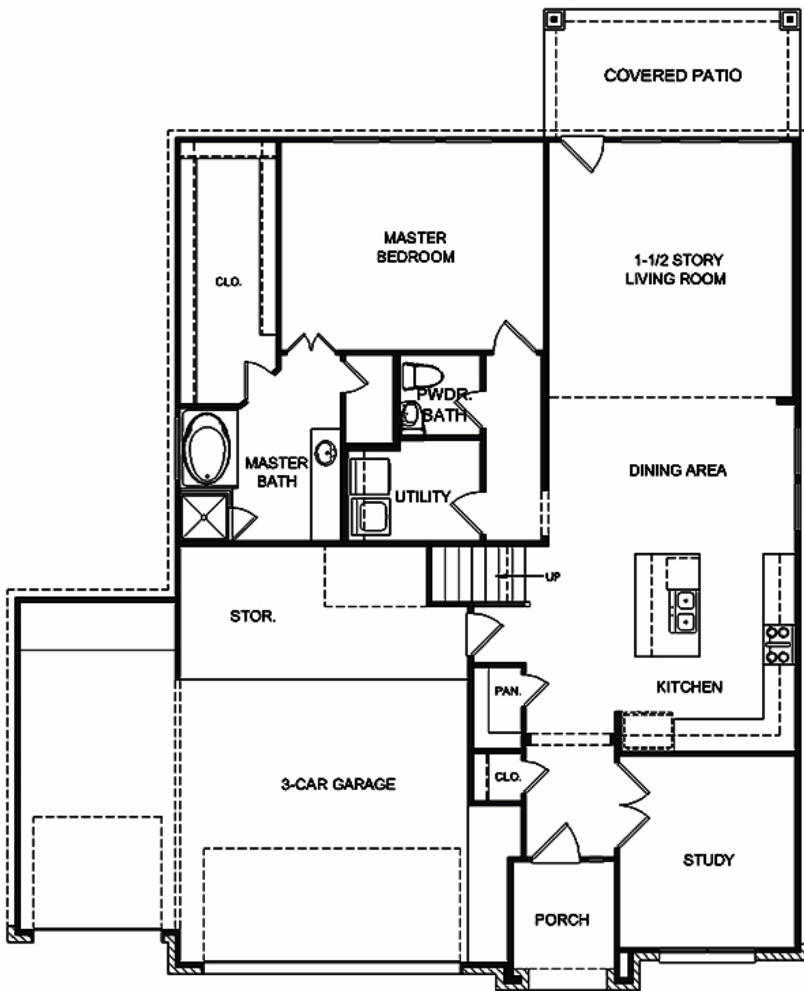
FIRST FLOOR PLAN PLAN 2377 3-CAR GARAGE
