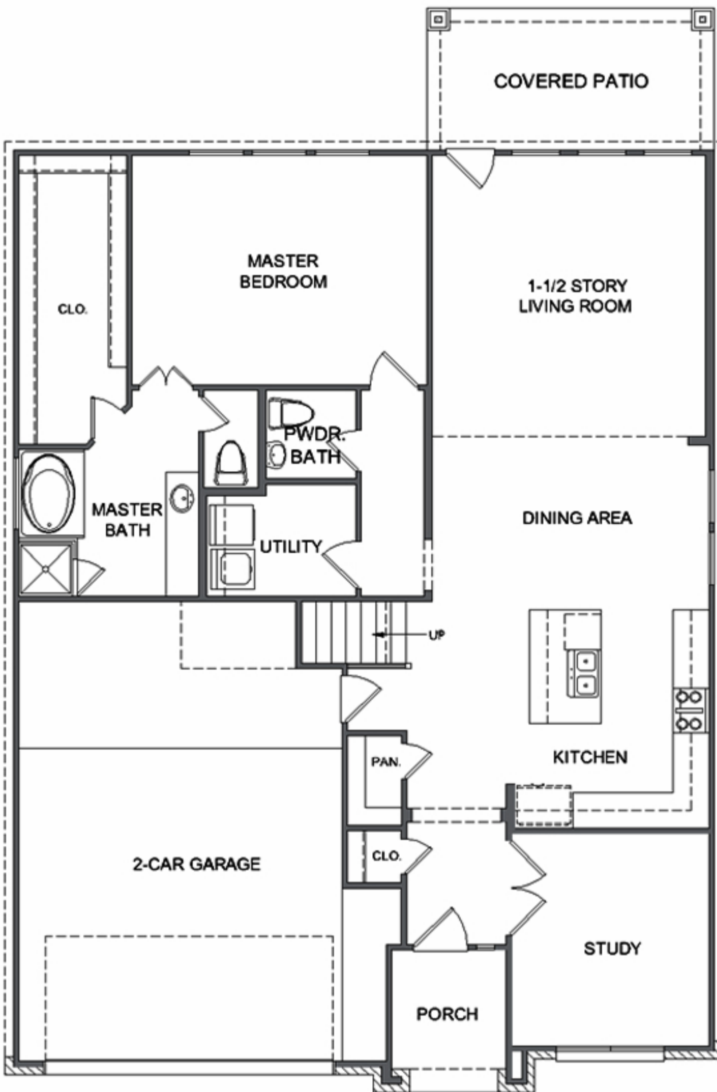
FIRST FLOOR PLAN PLAN 2377
