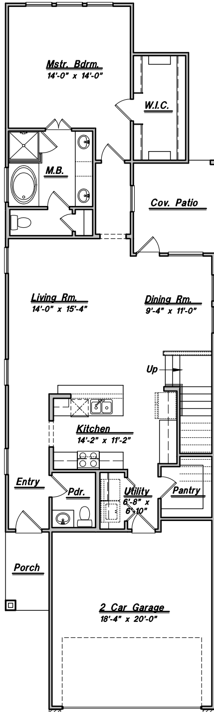
FIRST FLOOR Plan 2470
