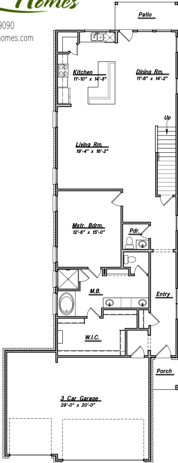
FIRST FLOOR Plan 2620
