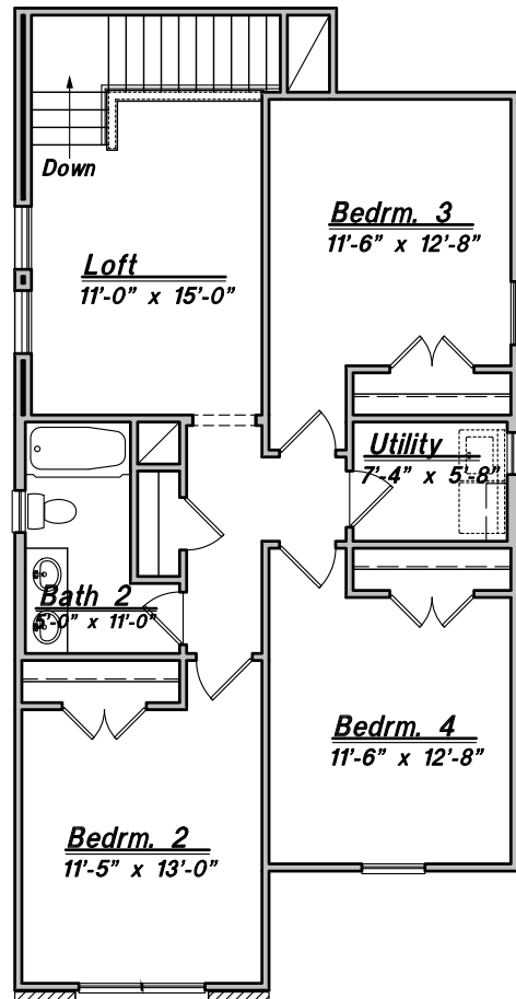
SECOND FLOOR PLAN 1860-ALT.
