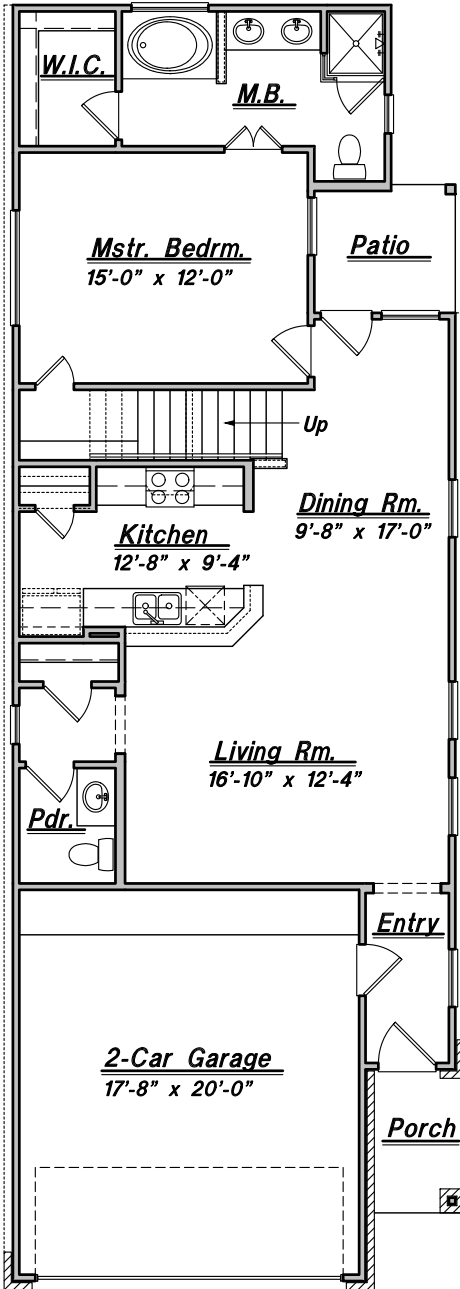
FIRST FLOOR PLAN 1860-ALT.
