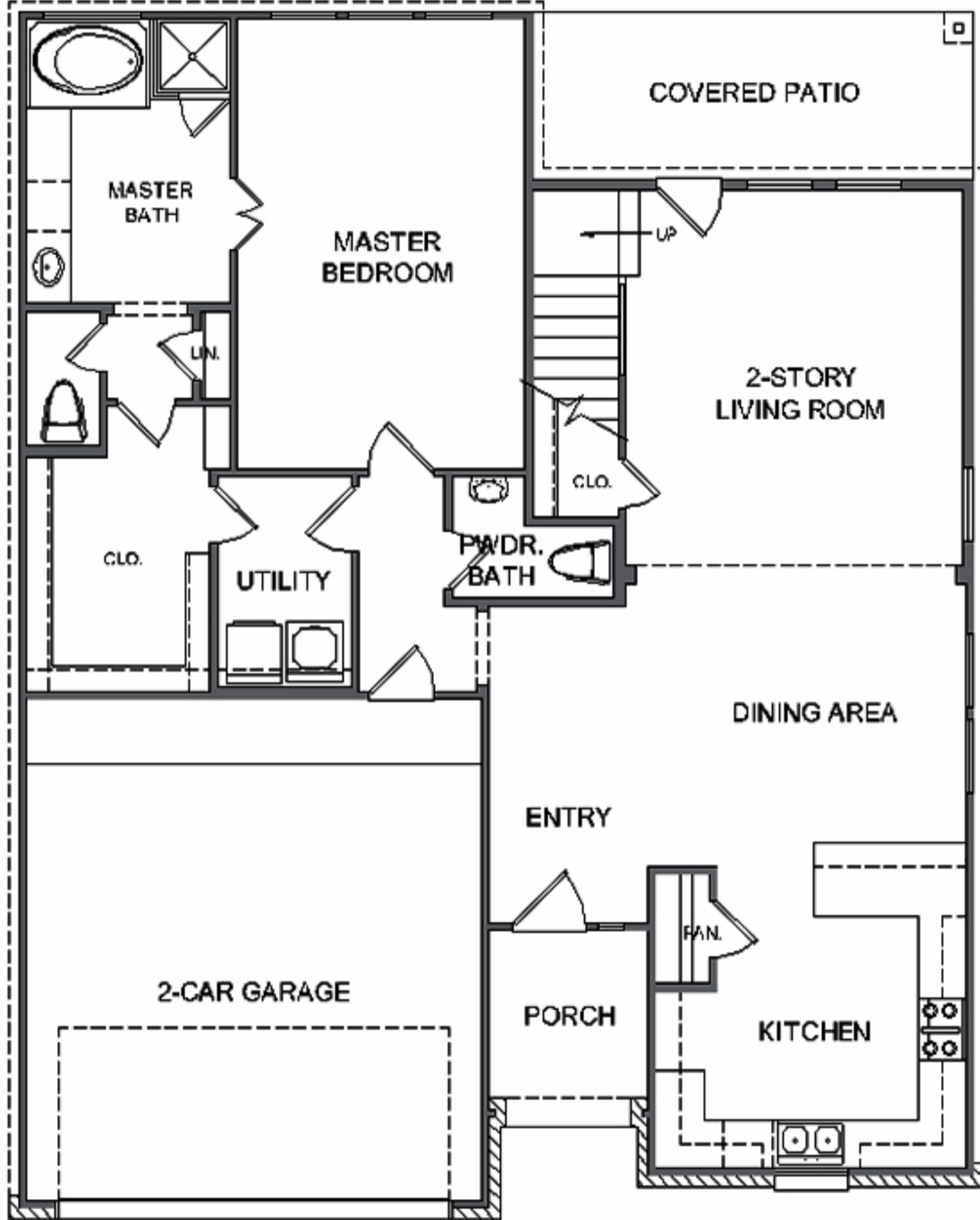
FIRST FLOOR PLAN PLAN 2365
