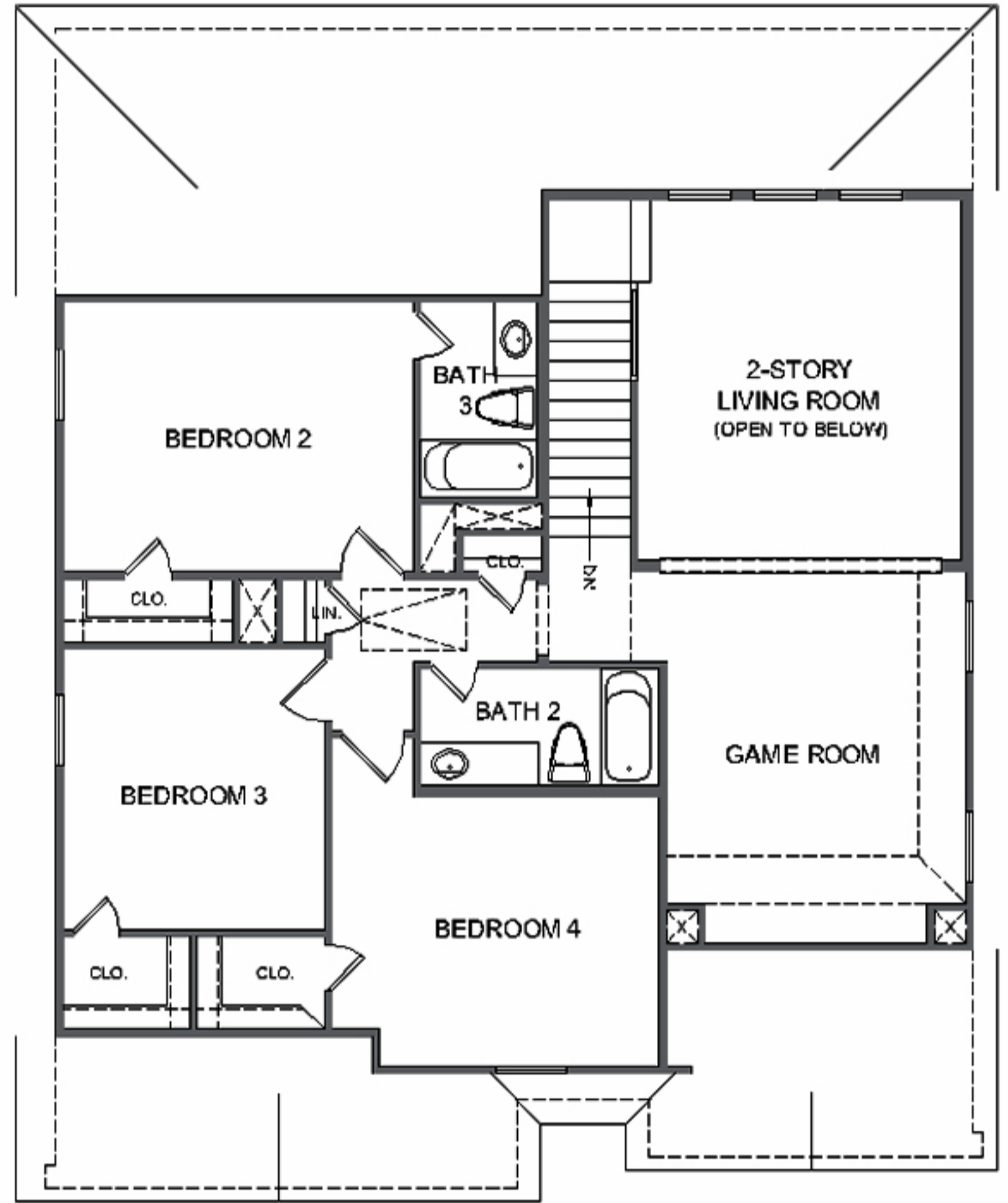
SECOND FLOOR PLAN PLAN 2365
